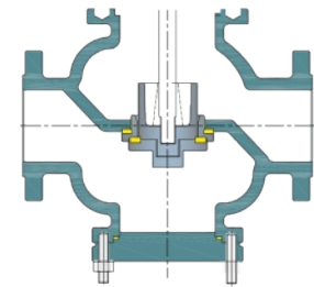
2/2 Way
